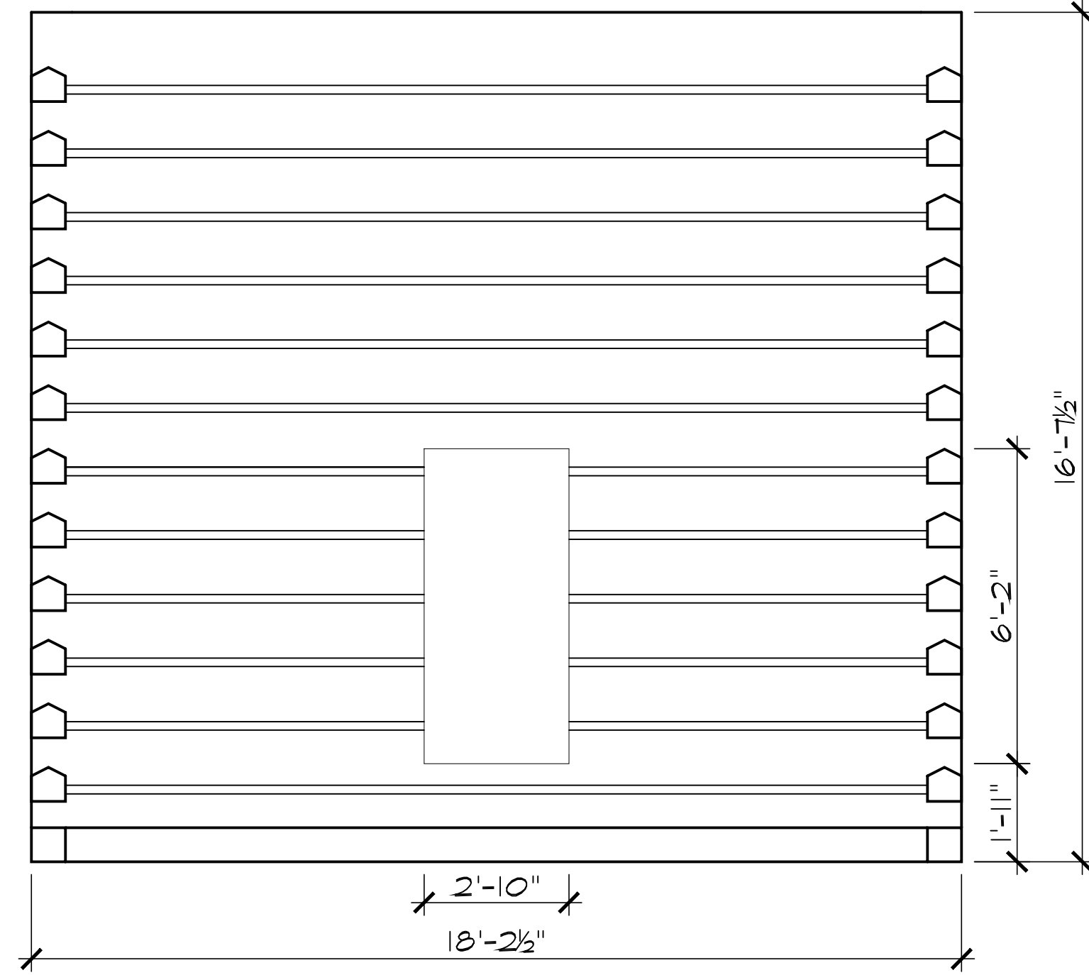
LEFT ELEVATION 3/8" = 1'-0"
