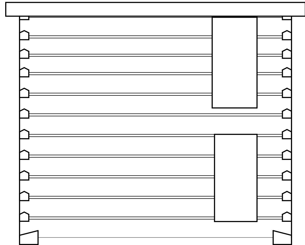
VIEW FROM TROT ELEVATION N.T.S.
